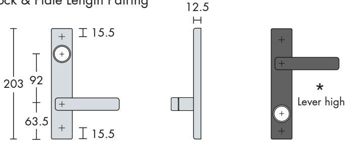
75 Series (172mm Fixing Centers) Accurate 9100 and similar USA mortise Locks
