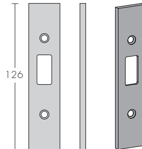
Mortise Latch Includes Magnetic Version 891
