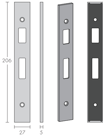
Mortise Lock Includes Magnetic Version 890
