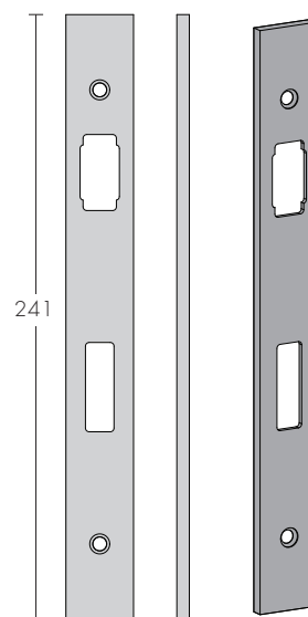
Mortise Roller Lock 893
